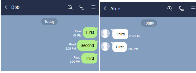
Figure 4: A MitM adversary blocks and reorders messages
