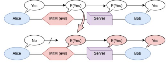
Figure 3: A replay attack in the MitM threat model of one-to-one communications. The MitM adversary replays Alice's first message. E(\text{Yes}) denotes an encryption of "Yes".
