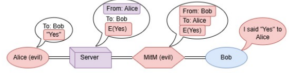
Figure 5: An impersonation attack under the threat model of a Malicious User colluding with the MitM adversary. Alice prepares a malicious message with honest metadata. The server infers the sender. The MitM maliciously alters the metadata.
