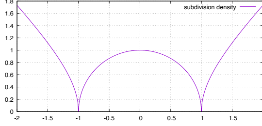
Fig. 6. Subdivision density for the parallel curve of an Euler spiral
