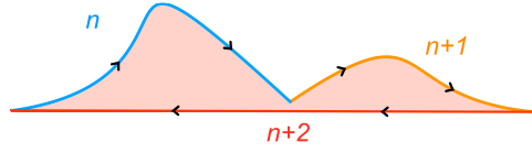
Fig. 13. Visualization of contour outlines and the IDs of GPU threads that flatten them. The subpath contains two adjacent cubic Bézier curves rendered as both a stroke and a fill. In the stroked version, thread n flattens the parallel curves of the first curve (blue) and the join segment with the miter style (dark blue). Thread n + 1 flattens the parallel curves of the second curve (orange) and the end cap with the round style (dark orange). Thread n + 2 handles the subpath end segment and flattens the start cap (red). When the same path is rendered as a fill, threads n and n + 1 each flatten the source curves, while thread n + 2 outputs the close segment that joins the end of the subpath to its starting point. The black arrows represent the winding direction of the output segments.
