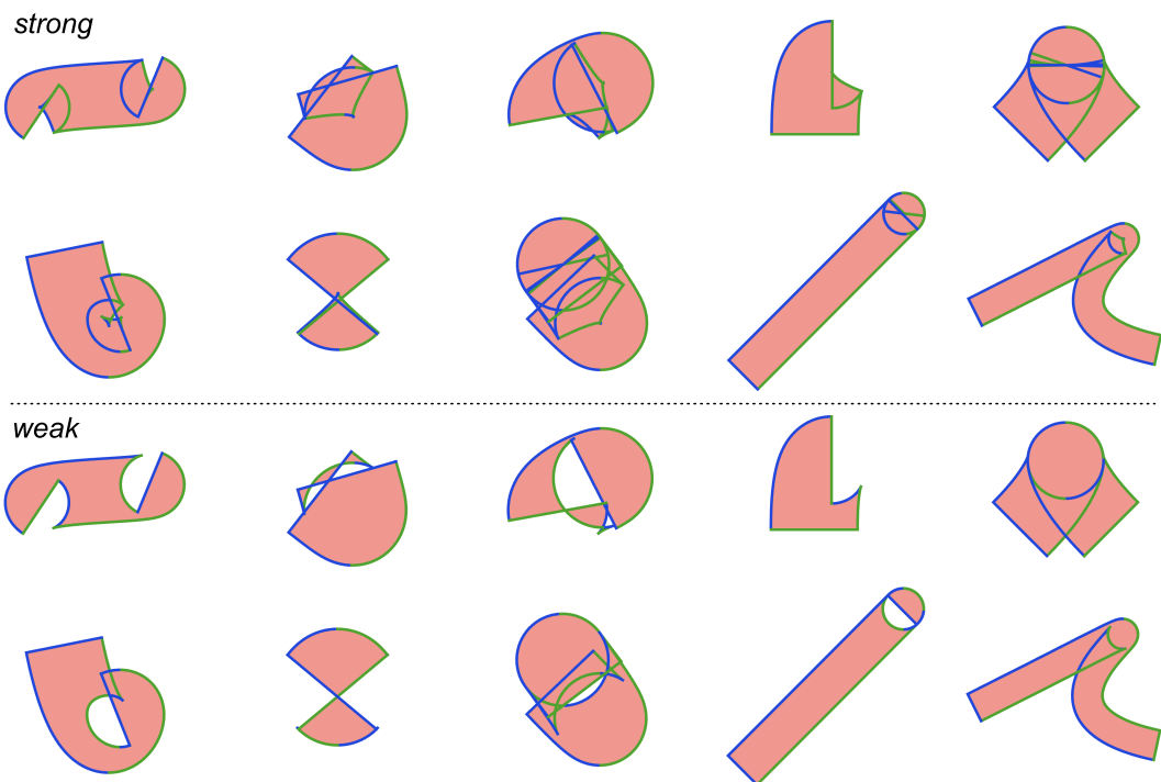
Fig. 12. Stroked cubic Béziels exhibiting strong and weak correctness, rendered by our implementation. The contents of the line soup buffer are visualized as green and blue outlines. Segments with a winding direction that points up are colored blue while those pointing down are colored green. The curves were adapted from the stills dataset by Nehab [2020] and the Skia test corpus.
