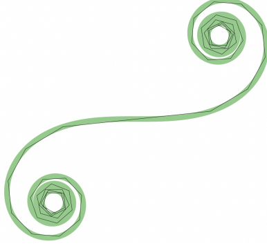
Fig. 4. The flattened approximation to an Euler spiral using line segments is achieved by choosing subdivision points using a simple power law formula with an exponent of 2/3 .
