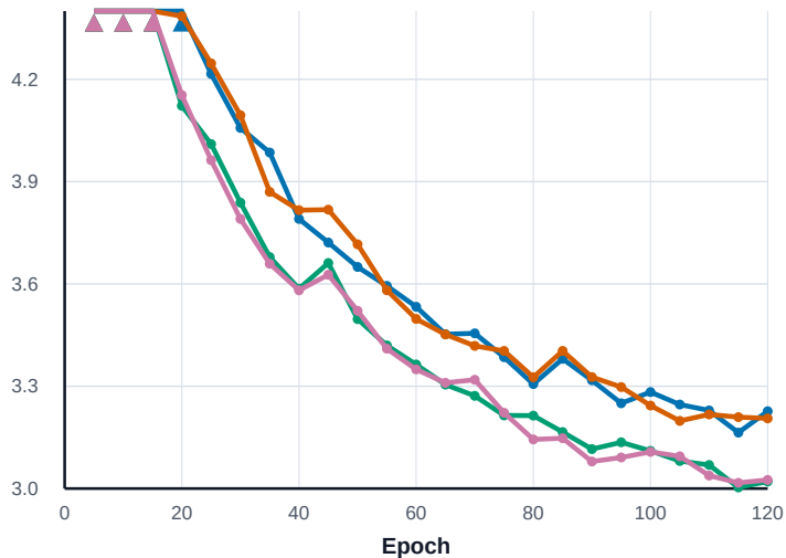
Mean EPE
