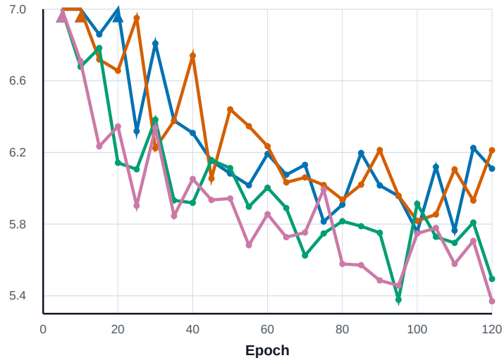
Sintel EPE
