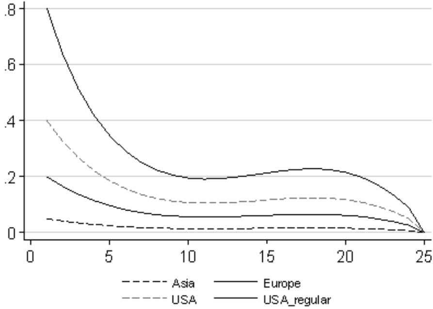
Figure 5.1 News impact decay structures \gamma_k(i)
