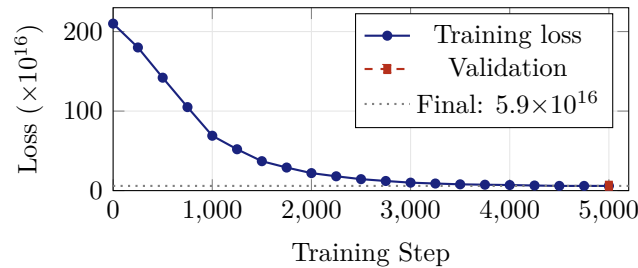
Figure 2: Training loss curve: 97% reduction ( 2.1 \times 10^{18} \rightarrow 5.9 \times 10^{16} ) in 5,000 steps / 43.4 minutes on a single GTX 1660 Ti. The loss plateaus after step 4,000, indicating convergence. Validation loss ( 6.1 \times 10^{16} ) is within 3.4% of training loss, confirming no overfitting.
