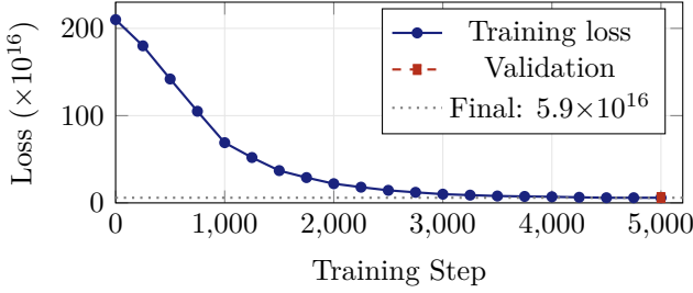
Figure 4: Training loss curve: 97% reduction ( 2.1 \times 10^{18} \rightarrow 5.9 \times 10^{16} ) in 5,000 steps / 43.4 minutes on a single GTX 1660 Ti. The loss plateaus after step 4,000, indicating convergence. Validation loss ( 6.1 \times 10^{16} ) is within 3.4% of training loss, confirming no overfitting.
