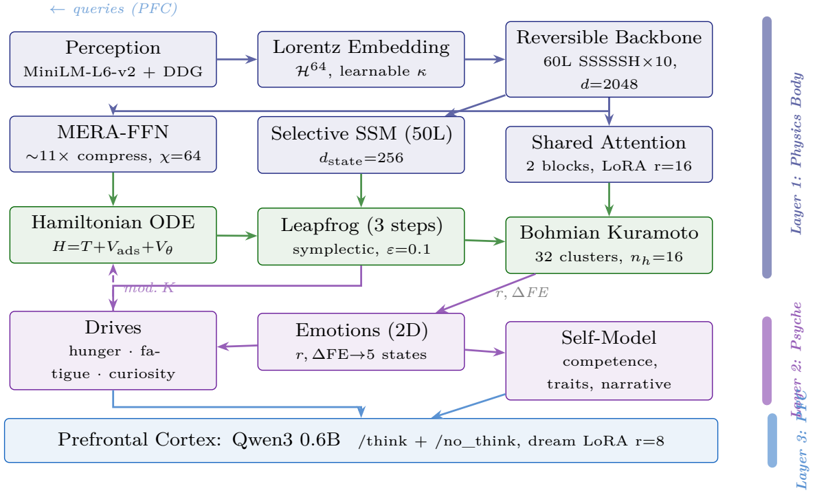
Figure 1: Three-layer architecture of Avatar 3.0. Blue: physics body processes perception through Lorentz embedding, MERA-compressed backbone, Hamiltonian dynamics, and Bohmian Kuramoto oscillators. Purple: psyche maps physics outputs ( r , \Delta FE ) to drives, emotions, and self-model. Dark blue: prefrontal cortex (Qwen3 0.6B) provides cognition and feeds queries back to perception. Solid arrows: forward data flow. Dashed arrows: feedback loops. Colored bars on right indicate layer boundaries.
