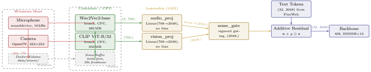
Figure 3: Multimodal sensory pipeline (v3.6). Raw audio and image signals are captured on the Windows host, written to a shared Docker volume, and read by frozen pretrained encoders inside the container. Learned SenseProjections gate and inject the encoded features as an additive residual into the text token stream. The physics body (backbone, Hamiltonian, Kuramoto) receives a unified multimodal representation in the Lorentz hyperboloid without any architectural change. Dashed boundaries indicate the host–container split.
