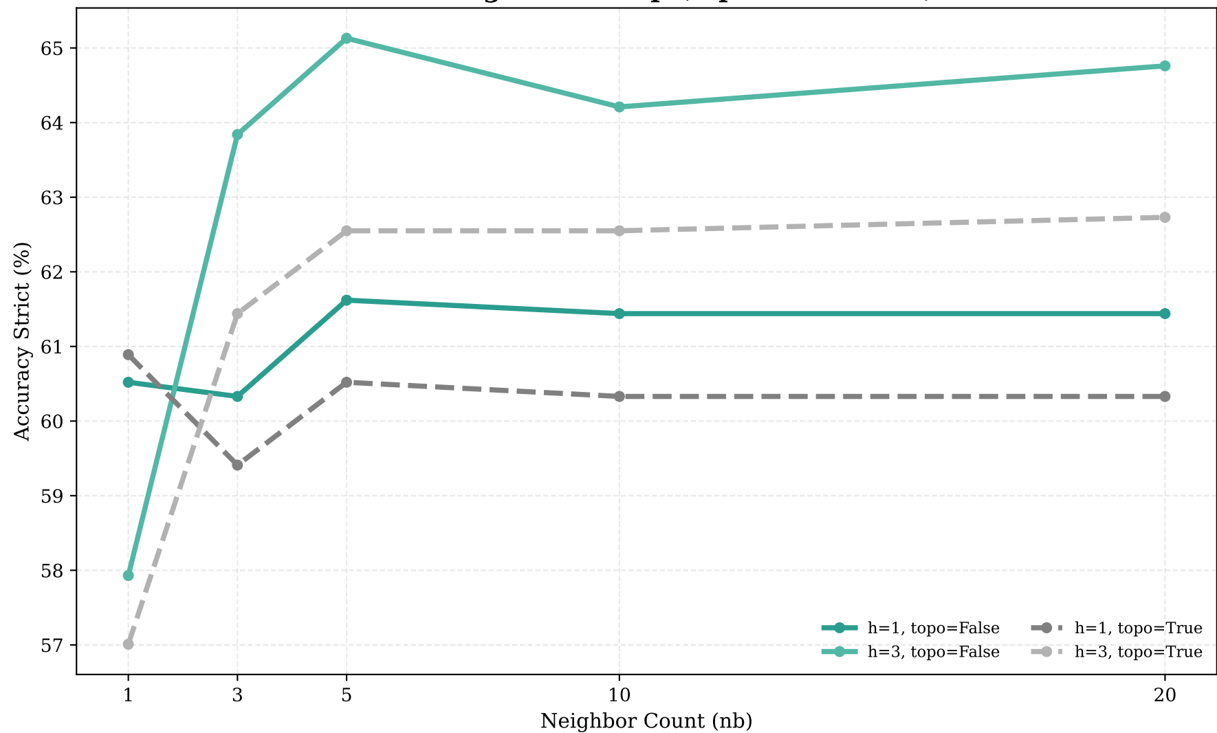
Cora Neighbor Sweep (topo=False/True)
