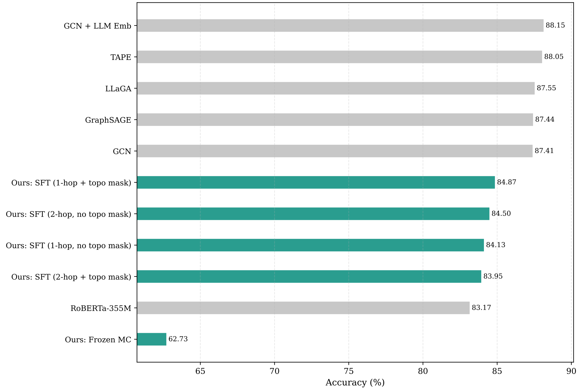
Cora Results (Bar)
