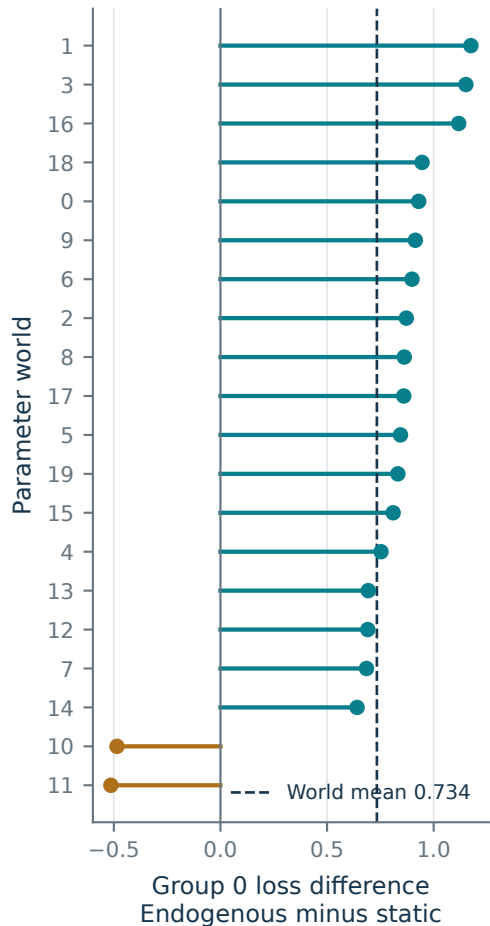
A All primary world effects
