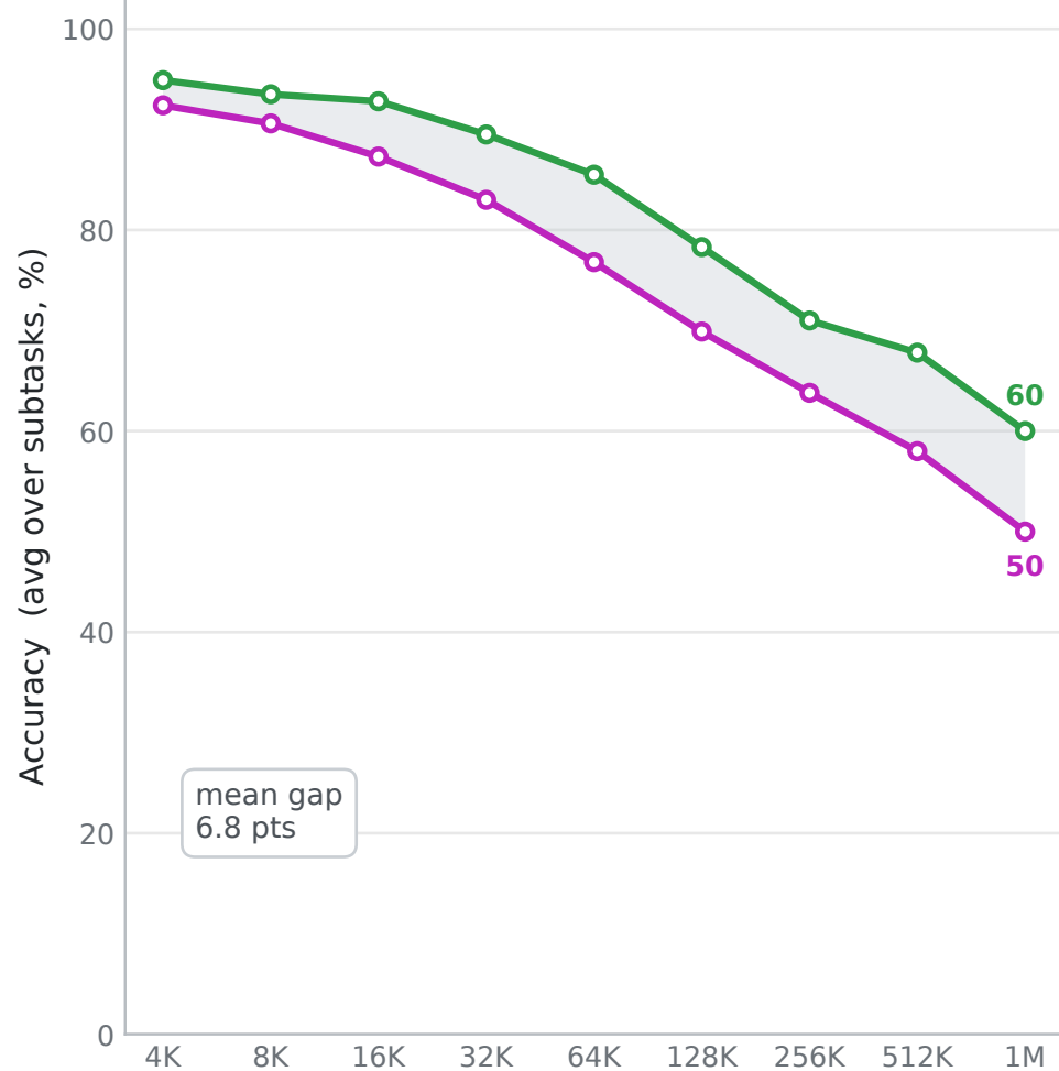
(a) Full RULER-13 · all 13 subtasks
