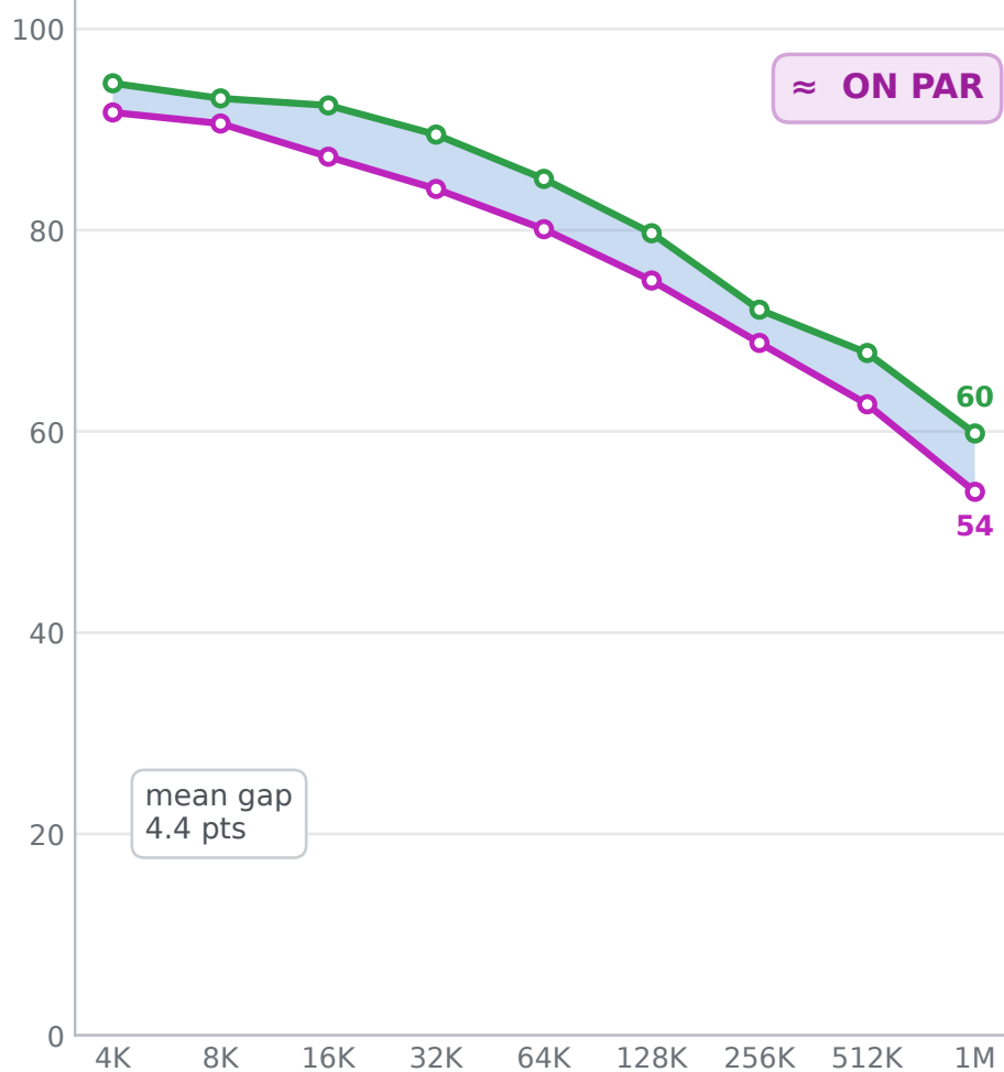
(b) RULER-13 excluding CWE
