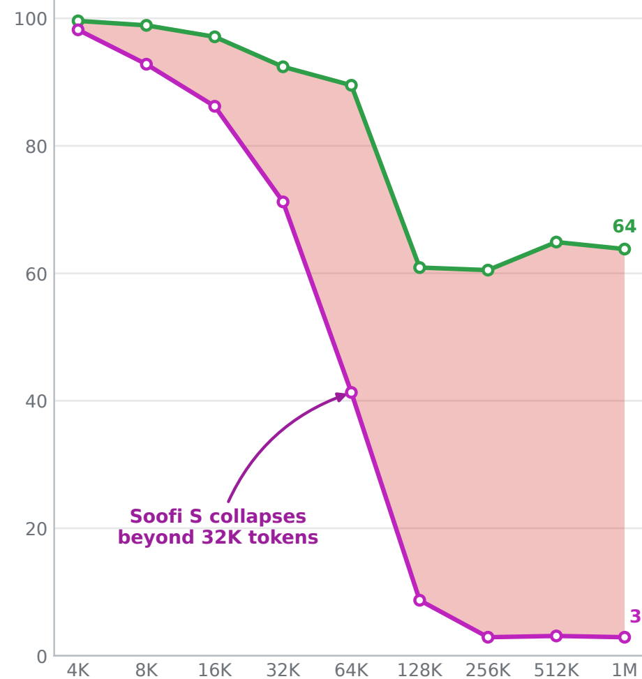
(c) CWE subtask only
