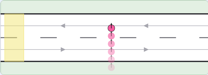
Jaywalker
