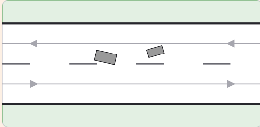
Road debris
