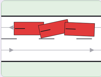
Collision: rear-end
