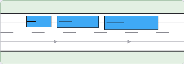
Parked vehicles
