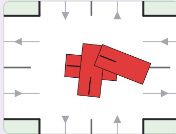
Collision: T-bone
