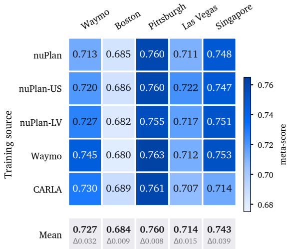
(a) WOSAC vehicle realism
