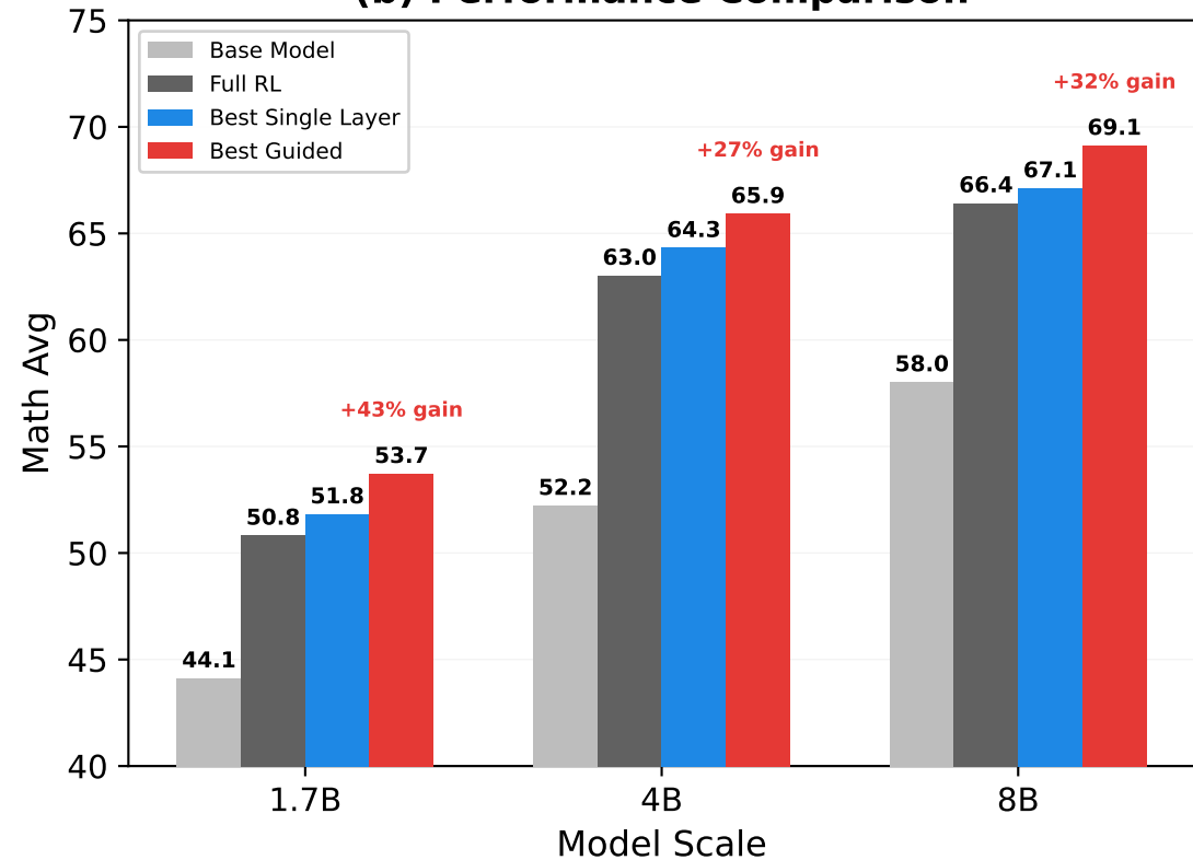
(b) Performance Comparison
