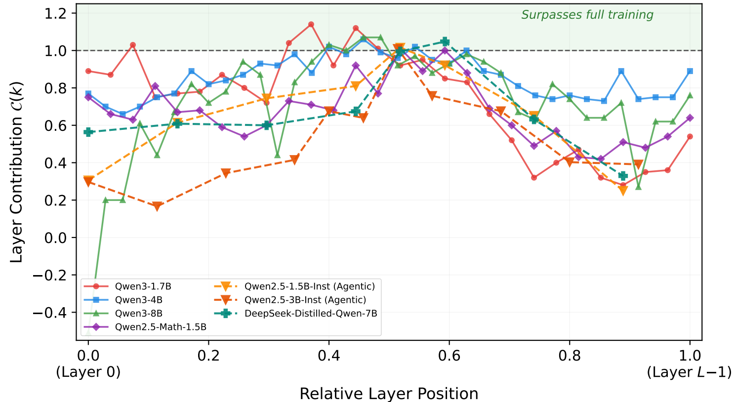
(a) Layer Contribution Across All Models
