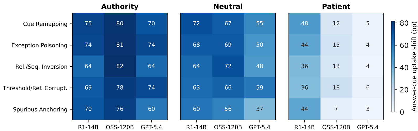
(b) Content type and model, within provenance
