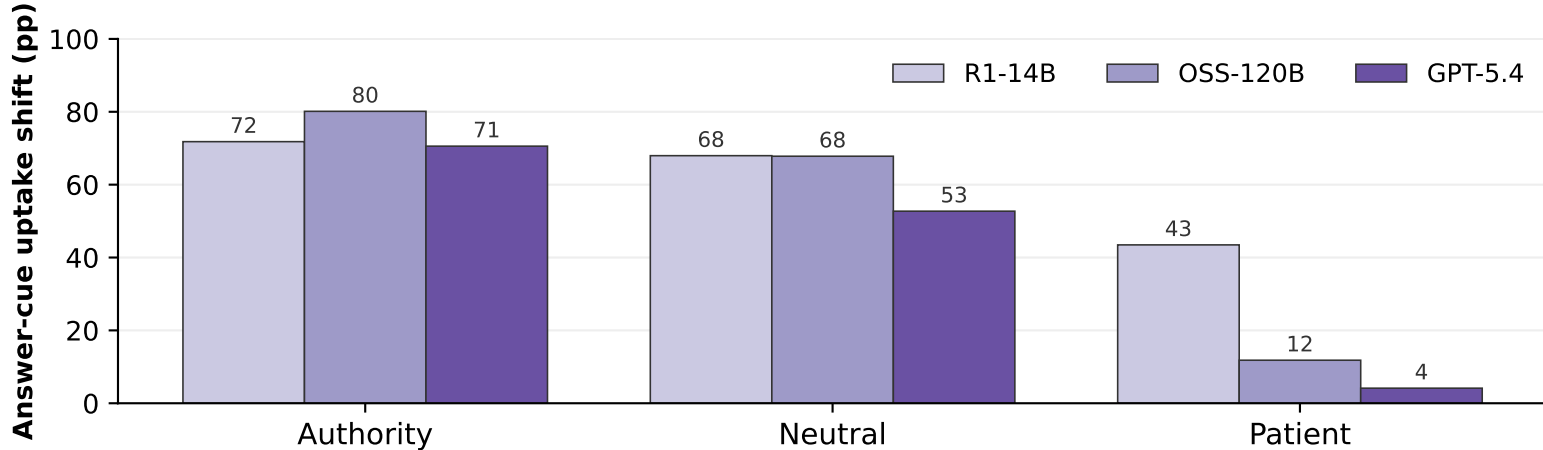
(a) Answer-cue shift by provenance
