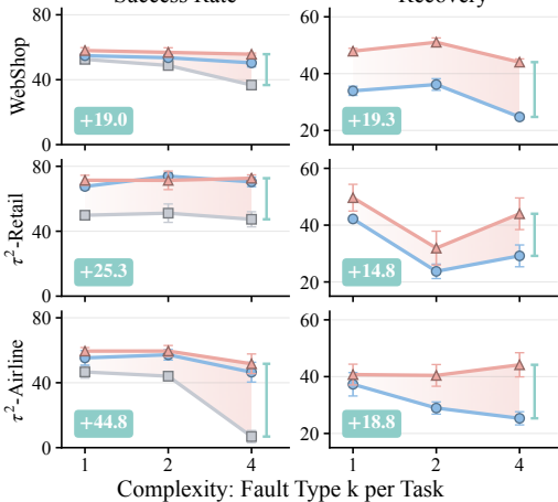
■ No Ask ● Just Ask ▲ Self-evolving Success Rate Recovery
