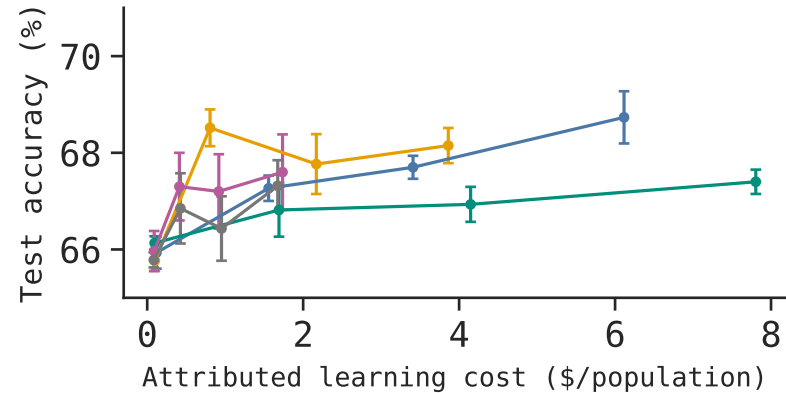
(a) GPT-0SS-120B
