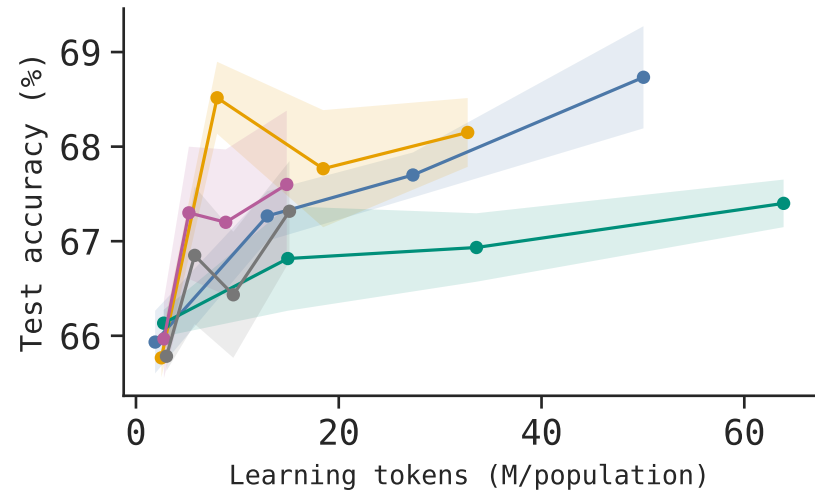
(a) GPT-0SS-120B
