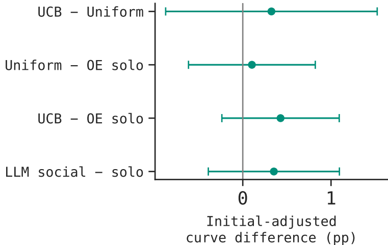
(a) GPT-0SS-120B
