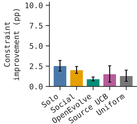
(c) GPT-OSS-120B
