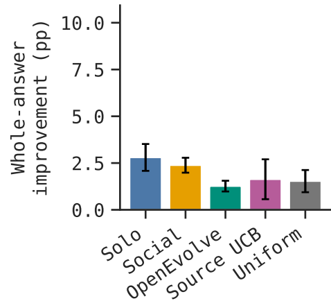
(a) GPT-OSS-120B
