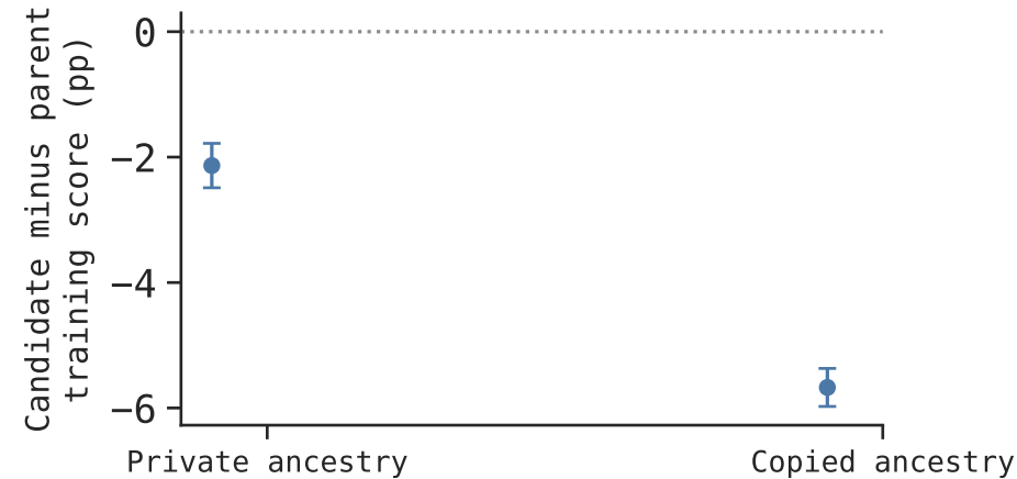
(a) GPT-0SS-120B
