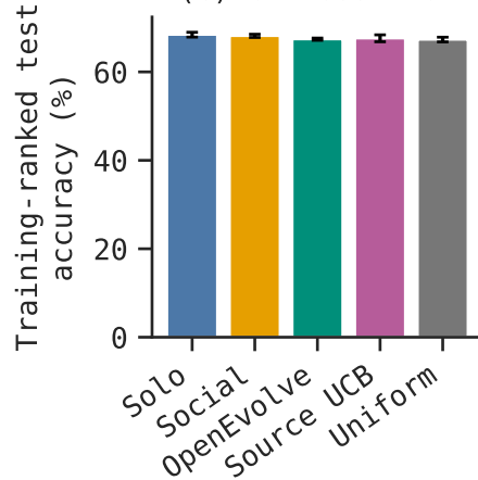
(c) GPT-OSS-120B
