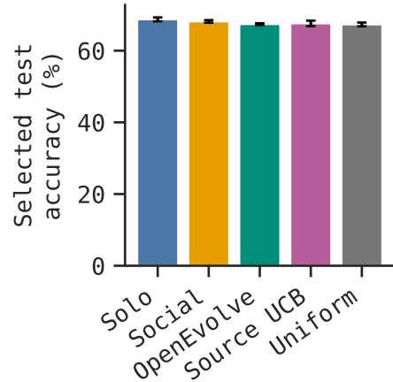
(a) GPT-OSS-120B
