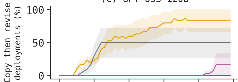
(c) GPT-0SS-120B
