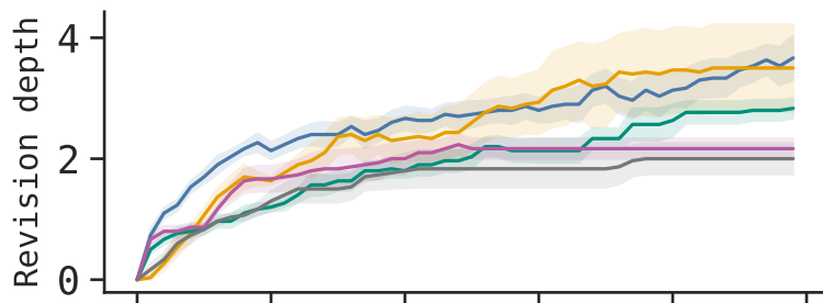
(a) GPT-0SS-120B
