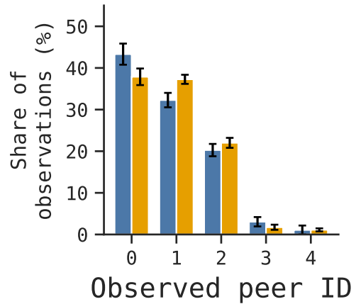
(a) GPT-OSS-120B
