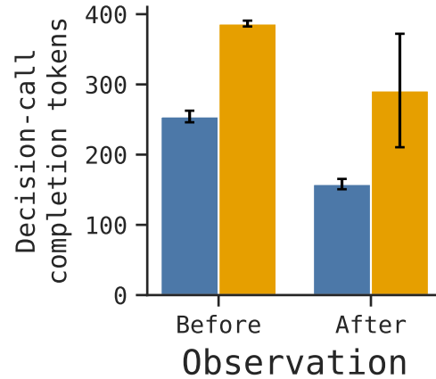
(c) GPT-OSS-120B
