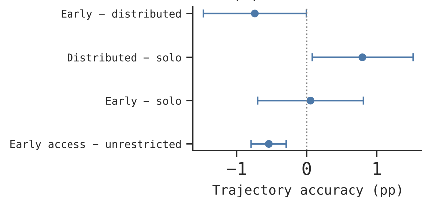
(c) GPT-OSS-120B
