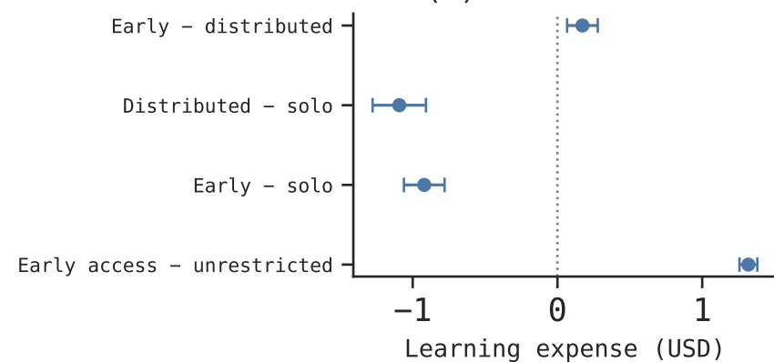
(e) GPT-OSS-120B
