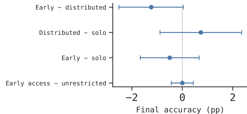
(a) GPT-OSS-120B
