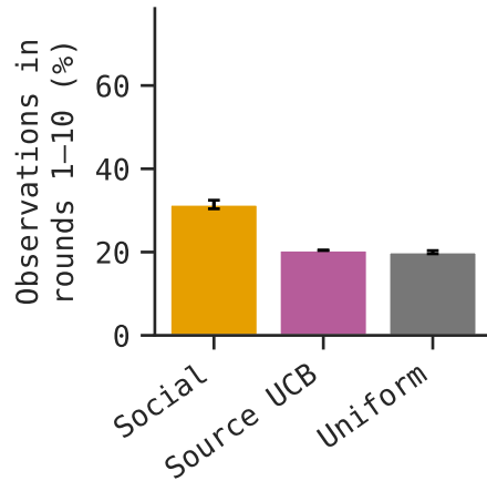
(c) GPT-0SS-120B
