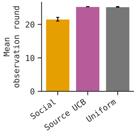
(a) GPT-0SS-120B
