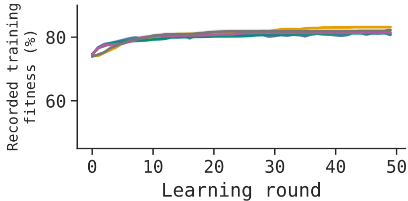
(a) GPT-0SS-120B
