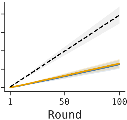
(c) Ministral
