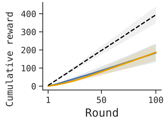
(a) Qwen
