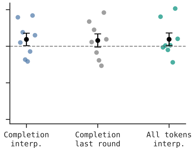
(b) Ministral-3-14B
