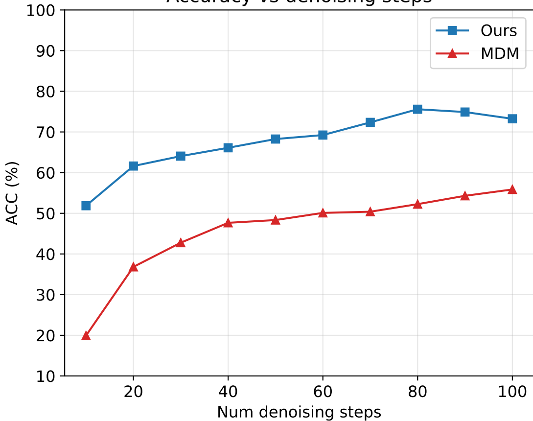
Accuracy vs denoising steps
