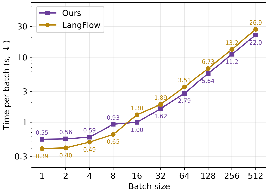
Sampling time per batch (NFE = 128, L = 128)
