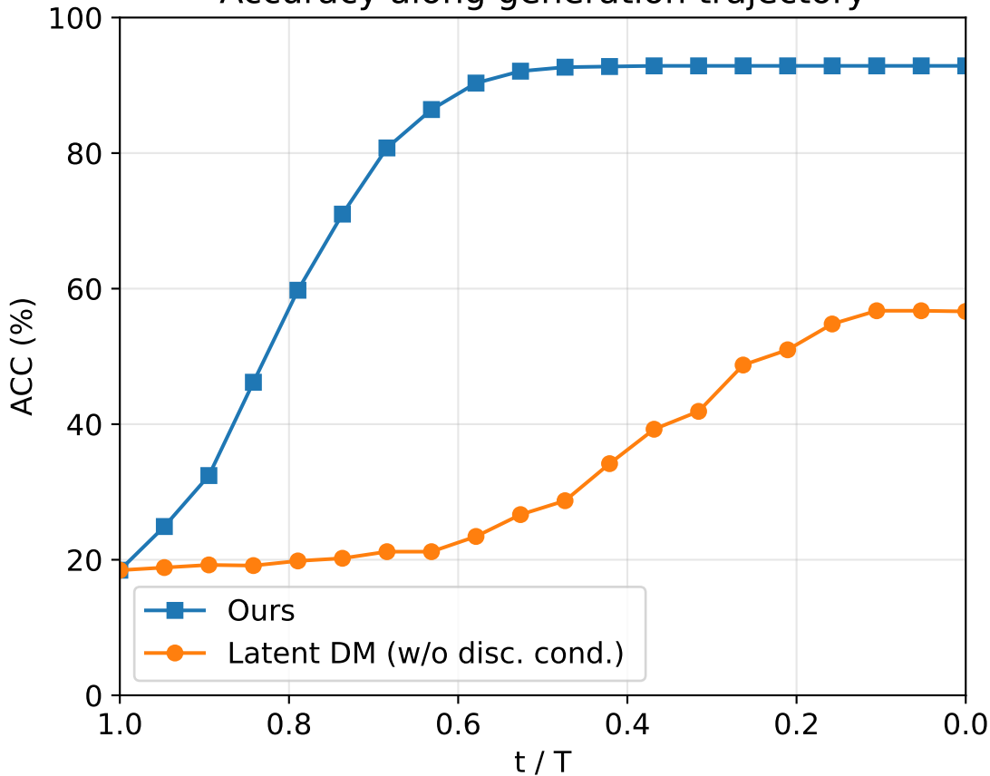
Accuracy along generation trajectory
