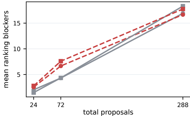
Infeasible sequences ranked ahead
