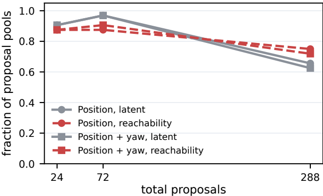
Feasible sequence remains in top 20
