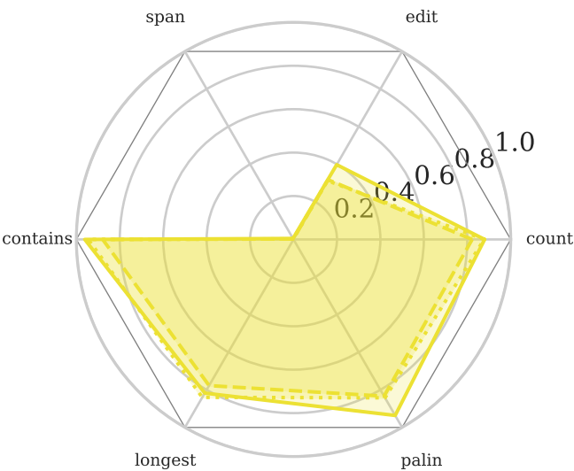
Qwen3.5-9 [NT]
