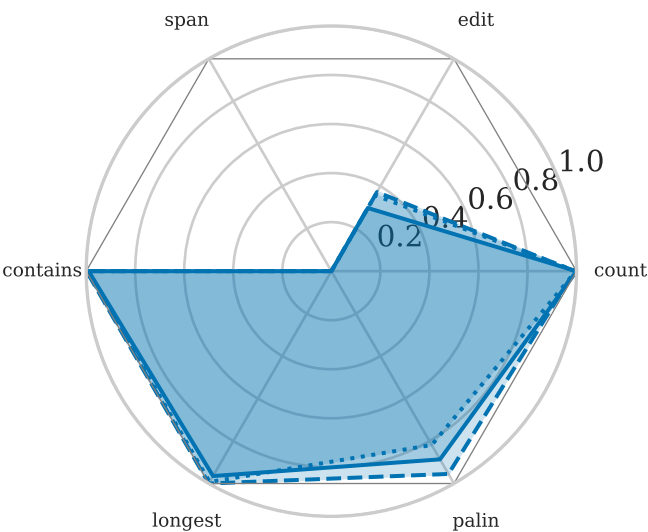
Qwen3.6-27 [T]
