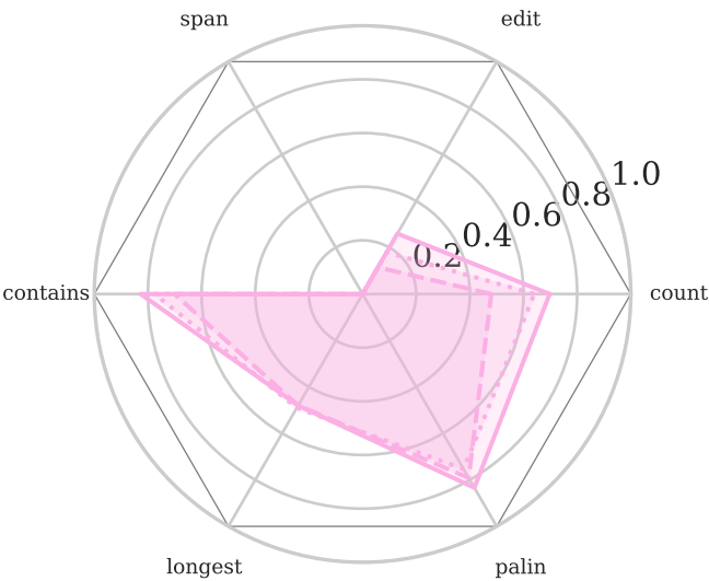
Qwen3.5-2 [NT]
