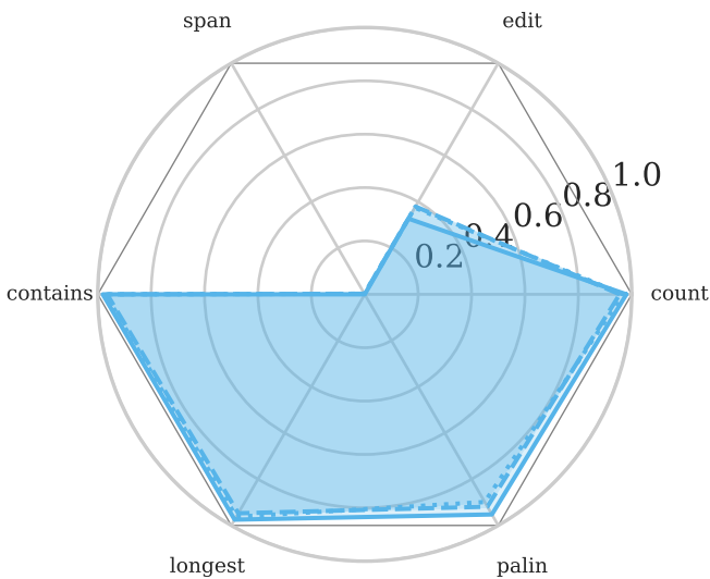
Qwen3.6-27 [NT]
