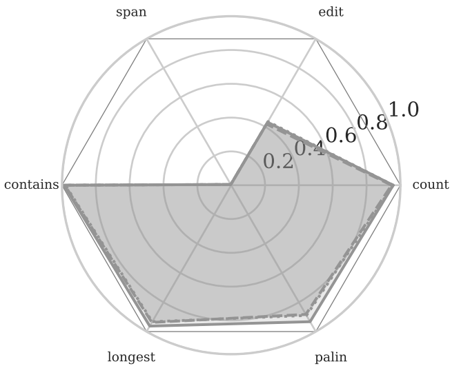
Qwen3.5-27 [NT]
