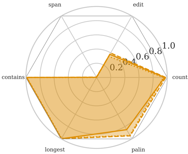
DeepSeek32 [T]
