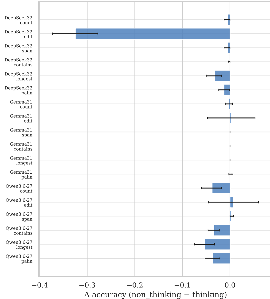
0-shot (paired samples)
