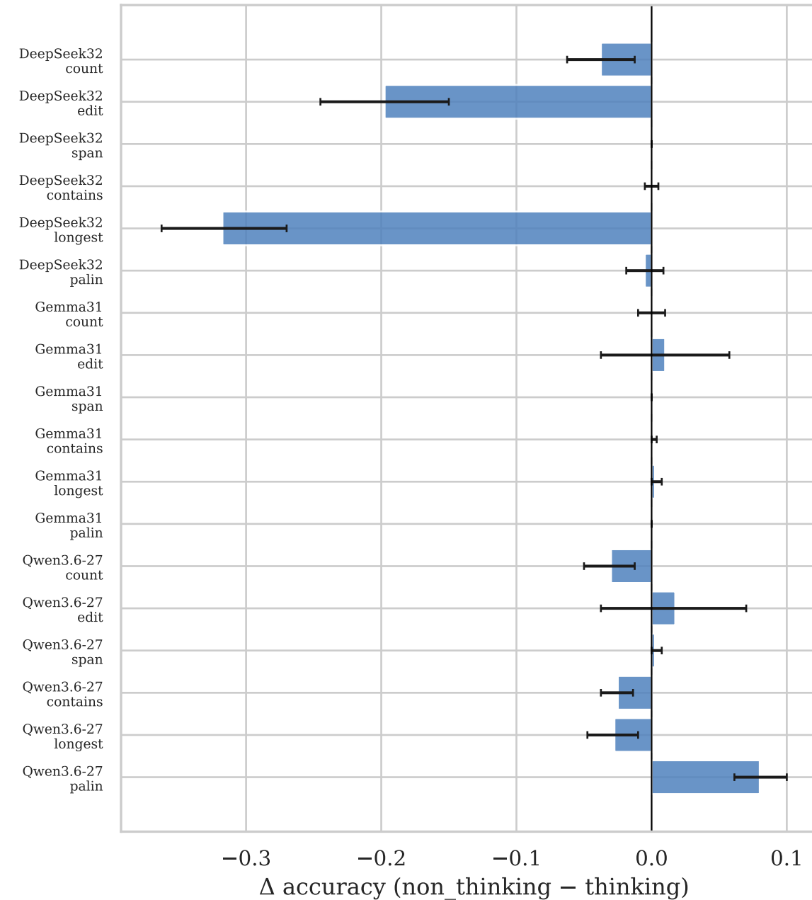
1-shot (paired samples)
