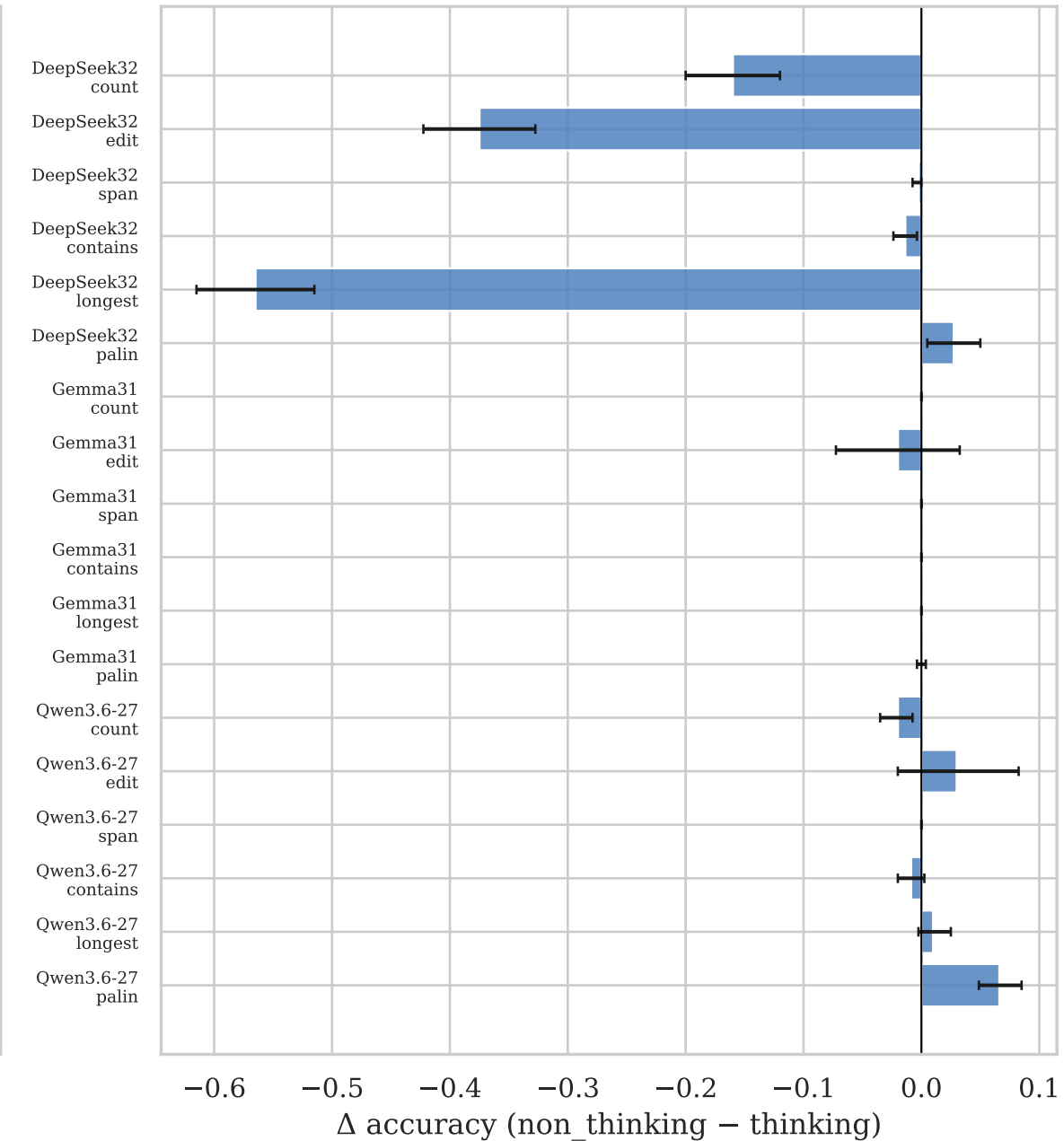
4-shot (paired samples)
