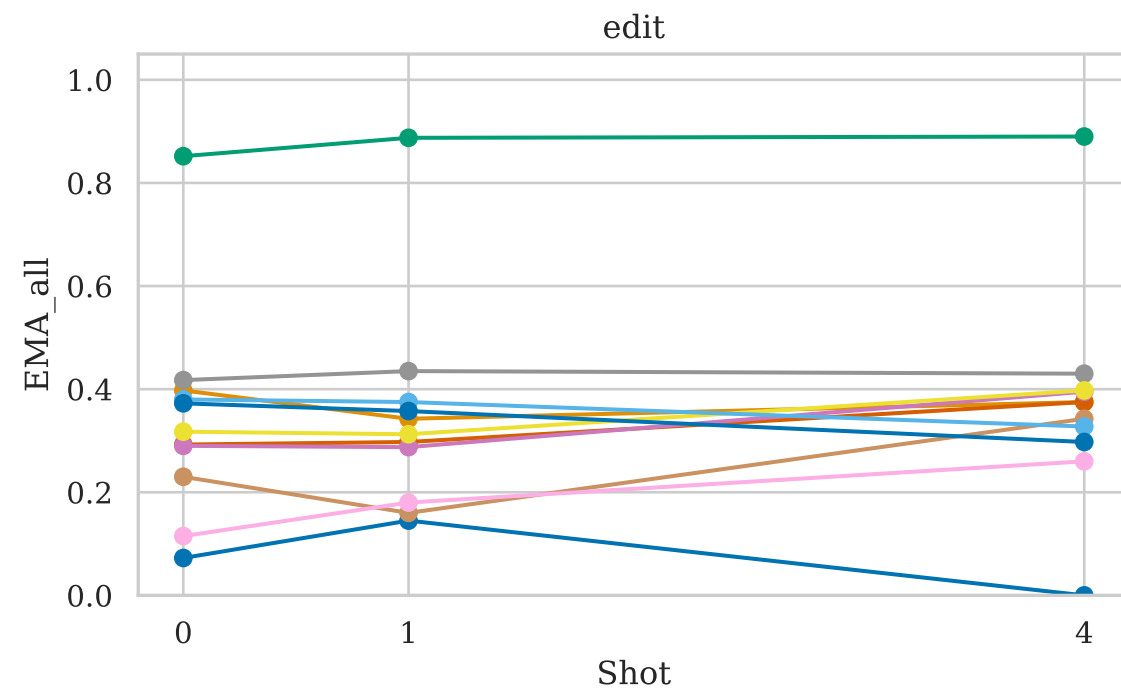
Shot-mode learning curves (condition=all)
