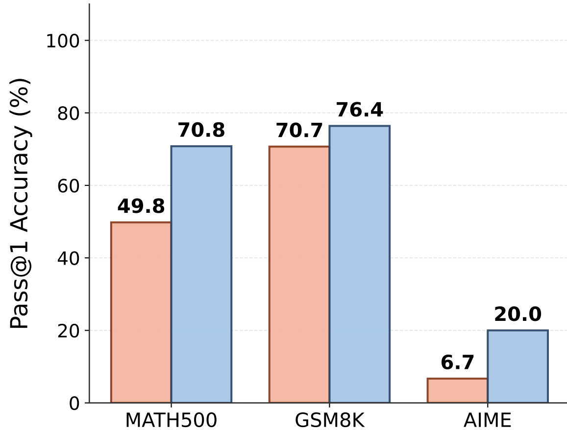
Reasoning Performance
