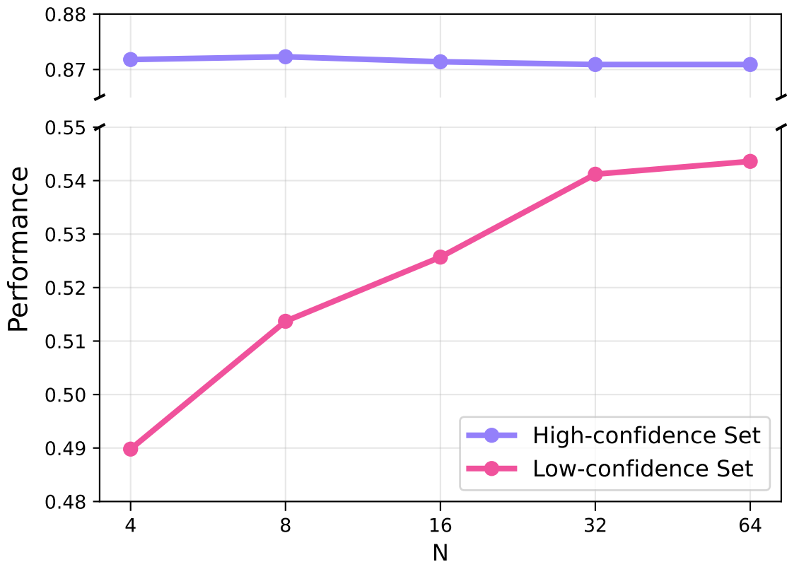
Different Benefits from Test Time Scaling for High-Confidence Set and Low-Confidence Set
