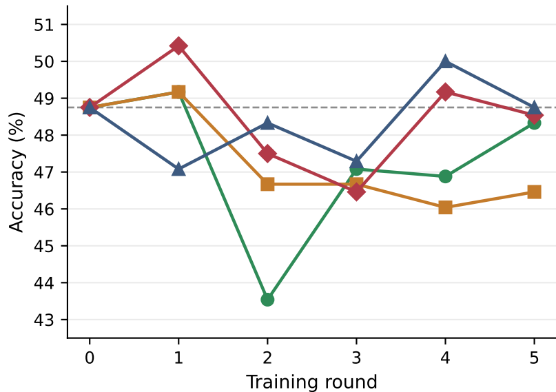
(c) Nemotron-Nano-8B · accuracy
