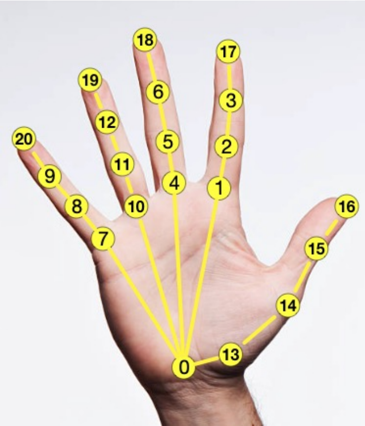
MANO keypoints
