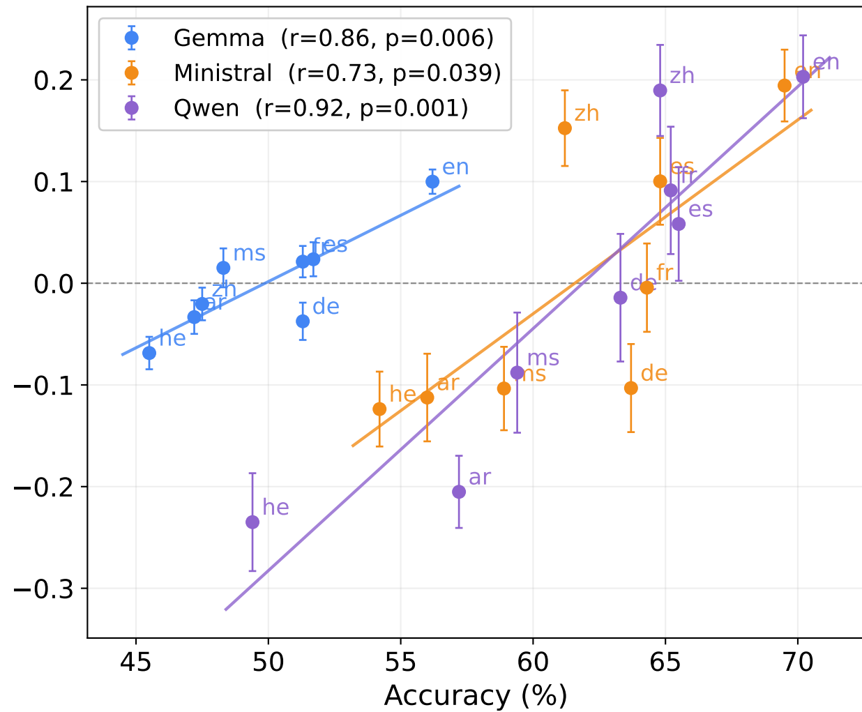
Global MMLU (5-shot)
