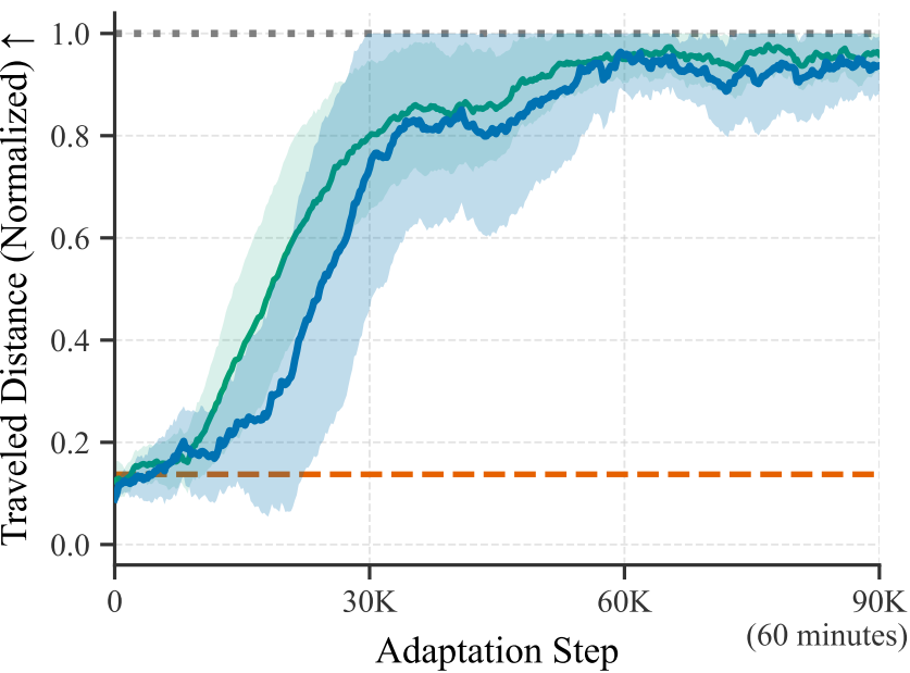
Planetary Traversal (Wheel Failure)
