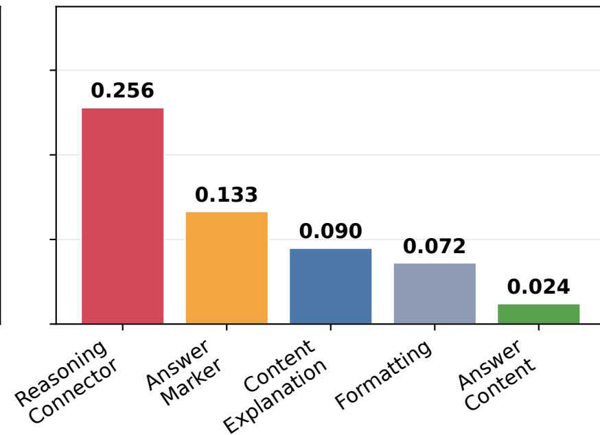
MATH-500
