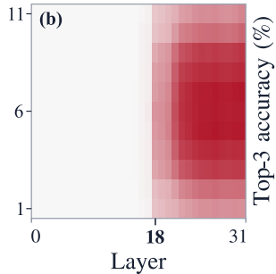
Steering using \bar{h}_D
