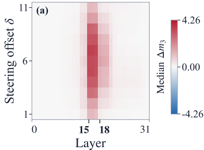
Steering using \bar{h}_\gamma
