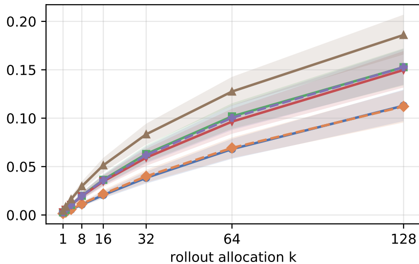
Omni-MATH 2 (OOD)
