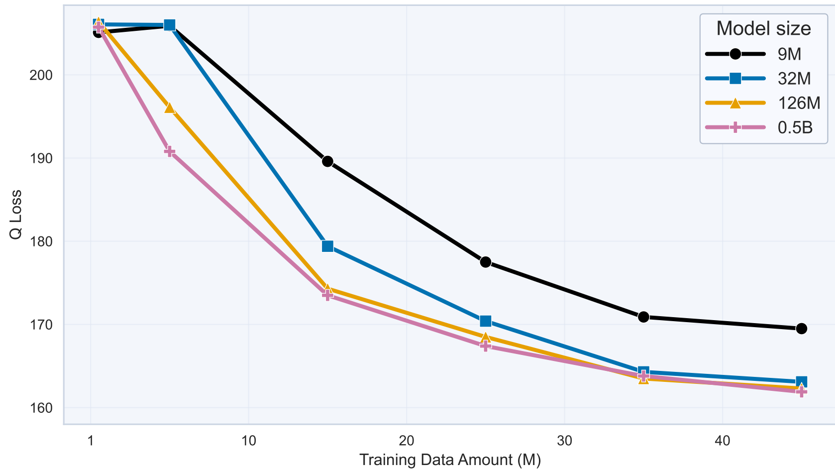
Q-Scaling Law Curves
