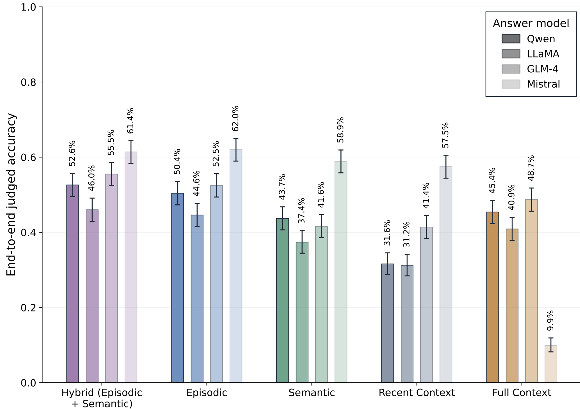
Overall accuracy (Gemma4)
