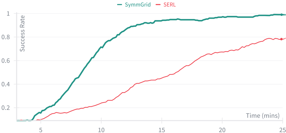
Real FR3 Cable-Routing Training Success Rate (Running Avg 50 Samples)
