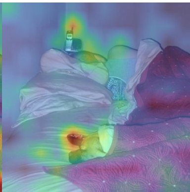
MMCS
