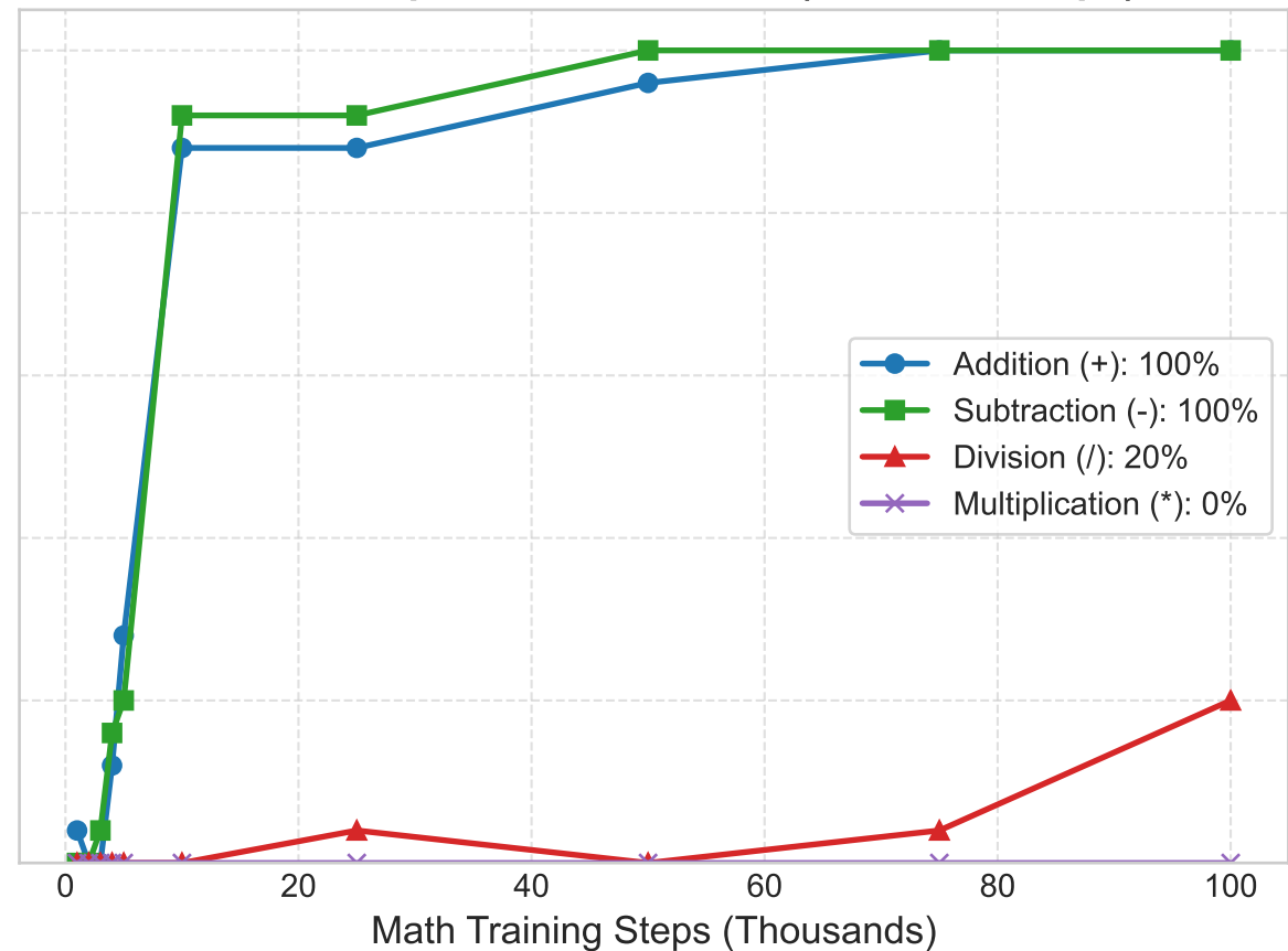
Run 8 Per-Operation Saturation (MoE 100k Steps)
