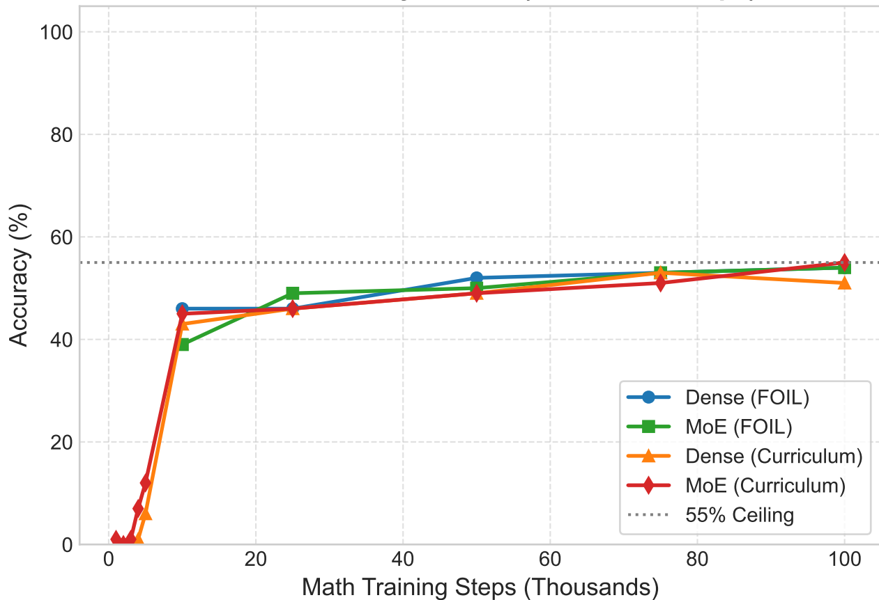
Overall Accuracy Plateau (10k to 100k Steps)
